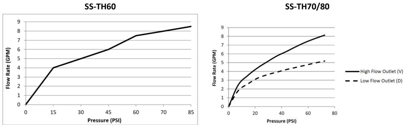
Diagram 1: Flow Rate Vs. Pressure
